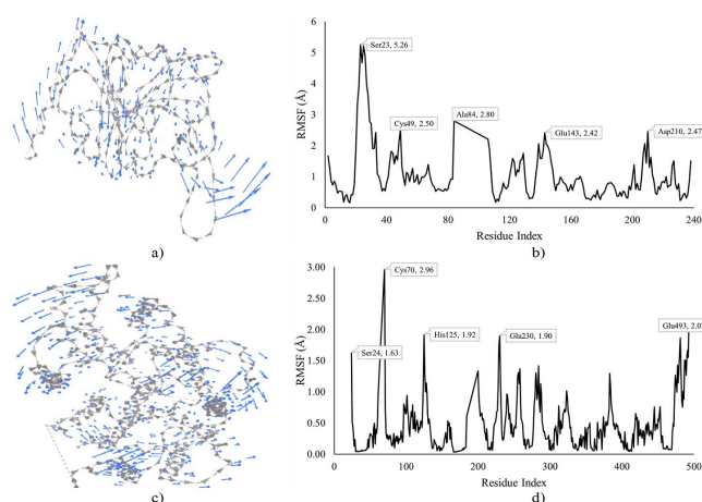
Figure 4. MDS of DHFRTS and PfHT1 docked with compound II and IV. Note: a) Cluster mobility of II with DHFRTS, b) RMSF of II with DHFRTS, c) Cluster mobility of IV with PfHT1, and d) RMSF of IV with PfHT1.
