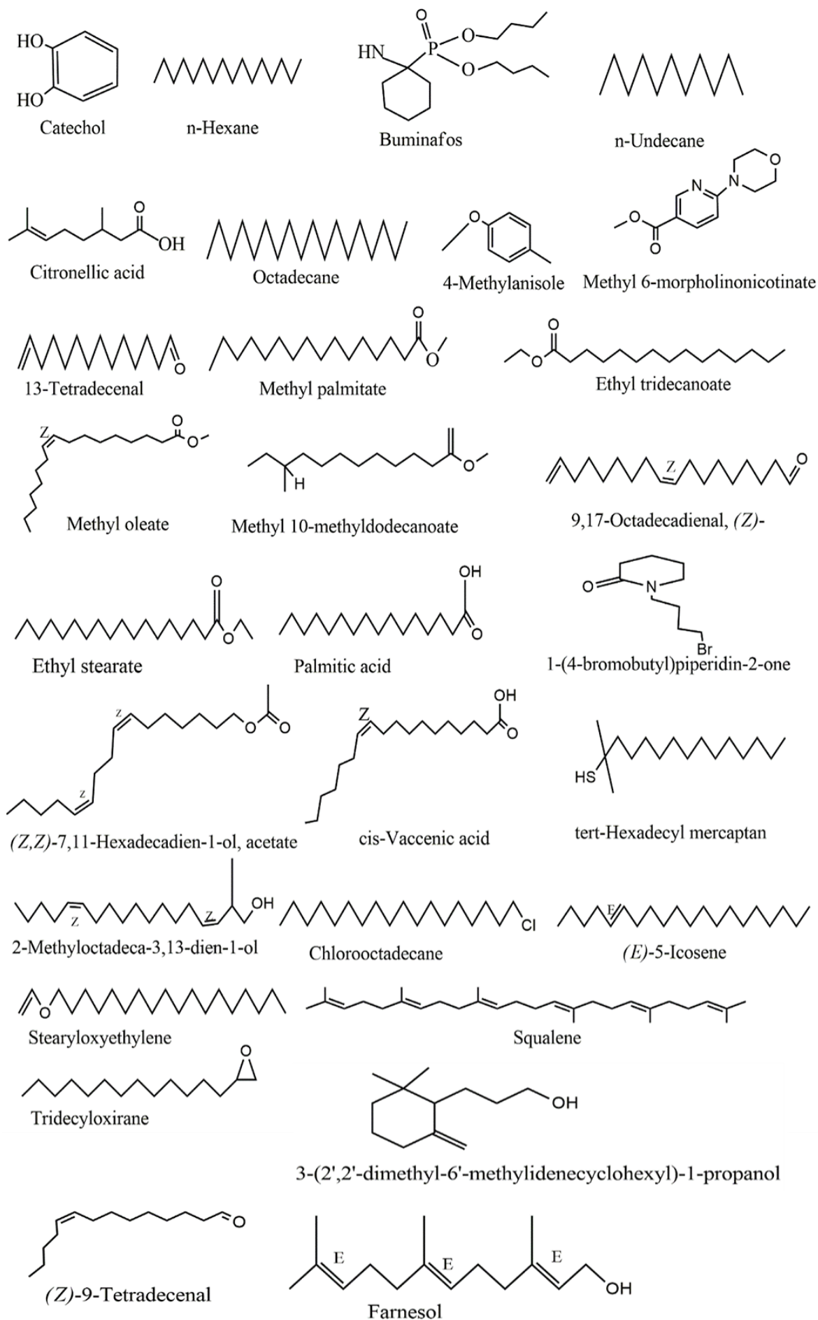
Figure 1. Structures of identified compounds in ethanol extract of Neonauclea excelsa .
