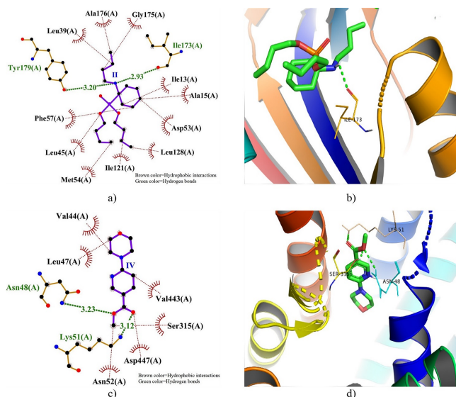
Figure 3. 2D and 3D docking interactions of DHFRTS and PfHT1 with compound II and IV. Note: a) 2D interaction of compound II with DHFRTS, b) 3D interaction of compound II with DHFRTS, c) 2D interaction of compound IV with PfHT1, and d) 3D interaction of compound IV with PfHT1.
