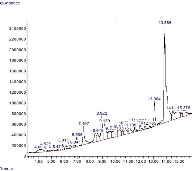
Figure 2. GC-MS Chromatogram of compounds identified in ethanol extract of Neonauclea excelsa .
