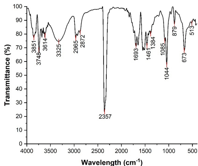
Figure 2. FTIR Spectrum for ethanolic extract of Sclerocarya birrea .
