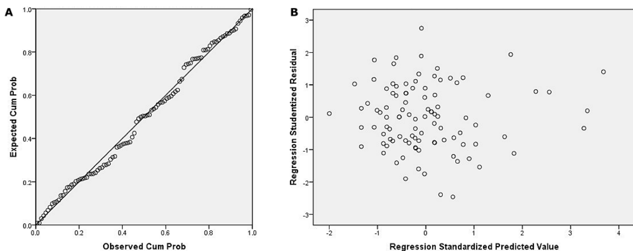
Figure 2. Model assumptions and diagnostic testing results. Note: (A) Normal P-P plot of regression standardized residual and (B) scatterplot of regression studentized residuals versus regression standardized predicted values.
